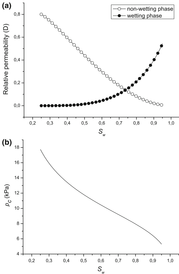
Fig. 5 Permeabilities (a) and capillary pressure (b) as a function of the wetting-fluid saturation
