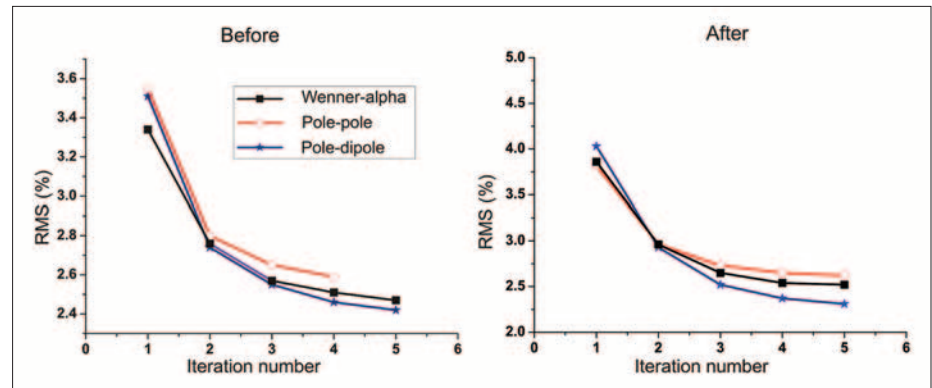
Figure 7. Plot of the rms errors versus number of iterations, before and after the CO 2 migration, for the different electrode configurations, where a = 1 m and n = 7 .
