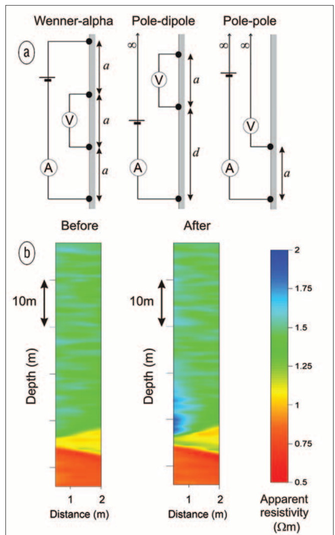
Figure 3. Representation of the electrode configurations (a) used in this work: Wenner-alpha, pole-dipole, and pole-pole, where a is the electrode spacing, n is the dipole spacing factor and d = na . The current is injected through the outer electrodes and measured by the amperometer A, while the potential is measured between the inner electrodes by the voltmeter V. Results of the forward modeling before and after the CO 2 migration using the pole-dipole configuration (b), where a = 1 m and n = 7 . It corresponds to the apparent resistivity of the medium, with 3% random noise added.
