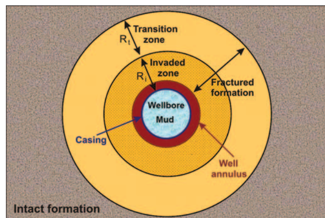
Figure 1. Planar section (not in scale) of the well and the surrounding medium, where R_i = 98 cm and R_t = 2 cm in the mudstone, and R_i = 97 cm and R_t = 3 cm in the sandstone.
