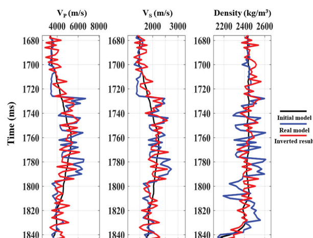
Figure 21. Comparison of the results in CDP121 shown in figure 18 with the well-log profiles of V_p , V_s and \rho in Well #2.
