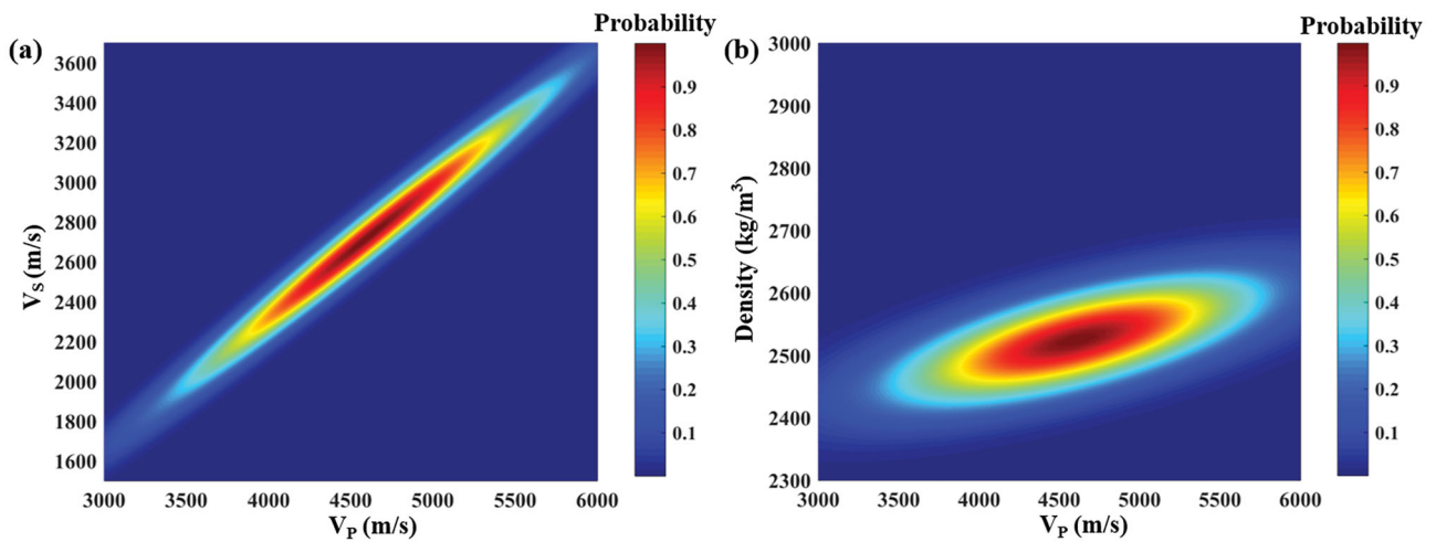
Figure 13. (a) V_p - V_s , (b) V_p -density multivariate Gaussian distribution prior probability for the limestone layer.
