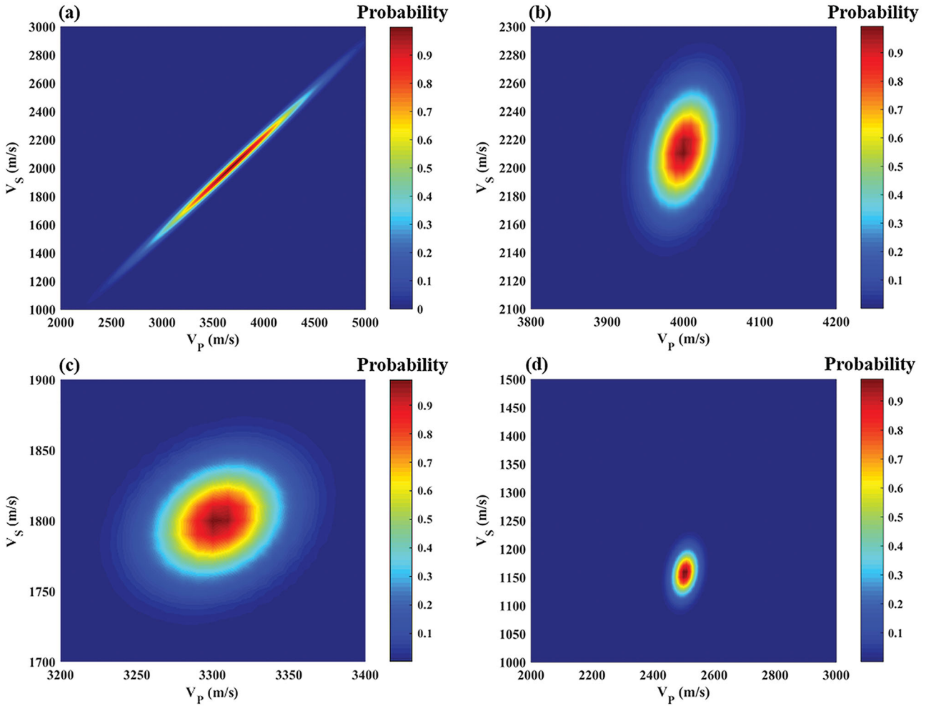
Figure 1. Multivariate Gaussian distribution prior probability of V_p and V_s for all layers (a), the shale layer (b), sandstone layer (c) and gas-sand layer (d).
