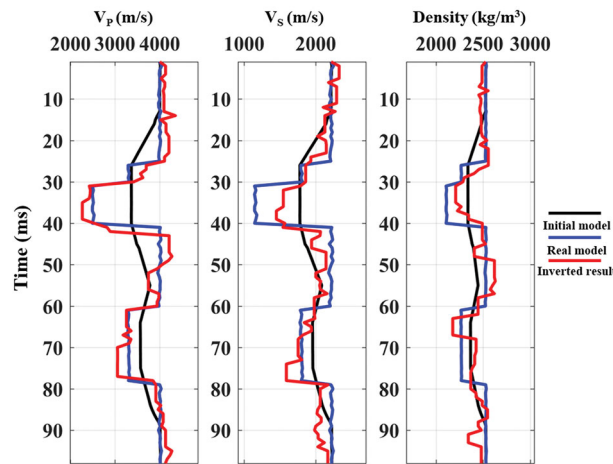
Figure 4. Results for V_p , V_s and \rho by conventional FSA algorithm without prior constraints.
